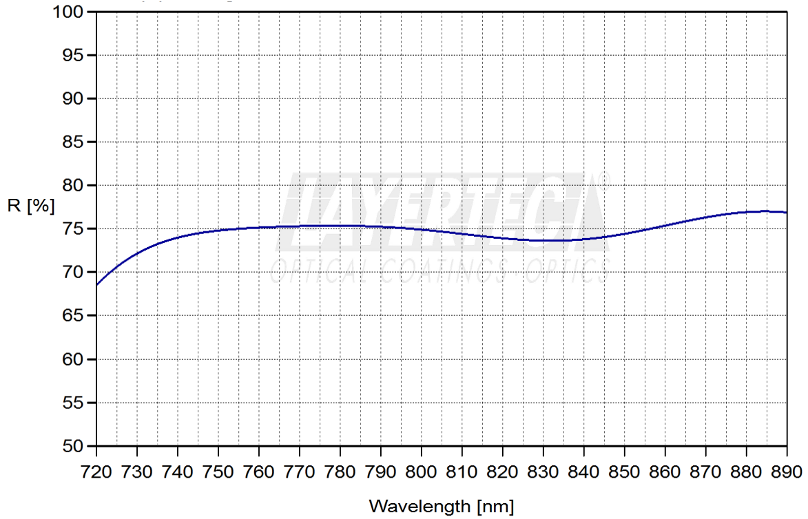
fig. 1.1: PRp (45°, 750-850nm) = 75 ± 2%
