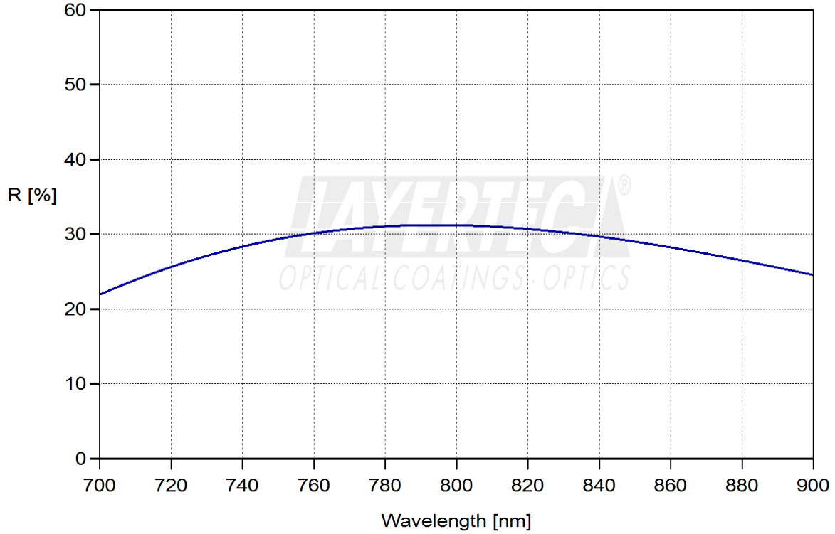
fig. 1.1: PRp (45°, 750-850nm) = 30 ± 3%
