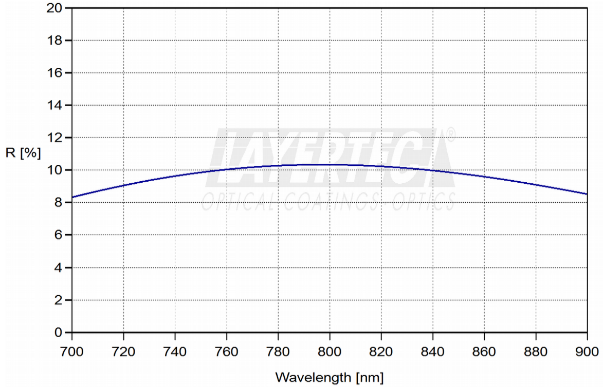
fig. 1.1: PRp (45°, 750-850nm) = 10 ± 3%
