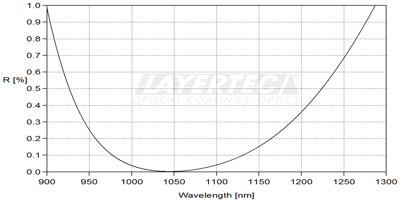
fig. 1 reflection AR 0°
