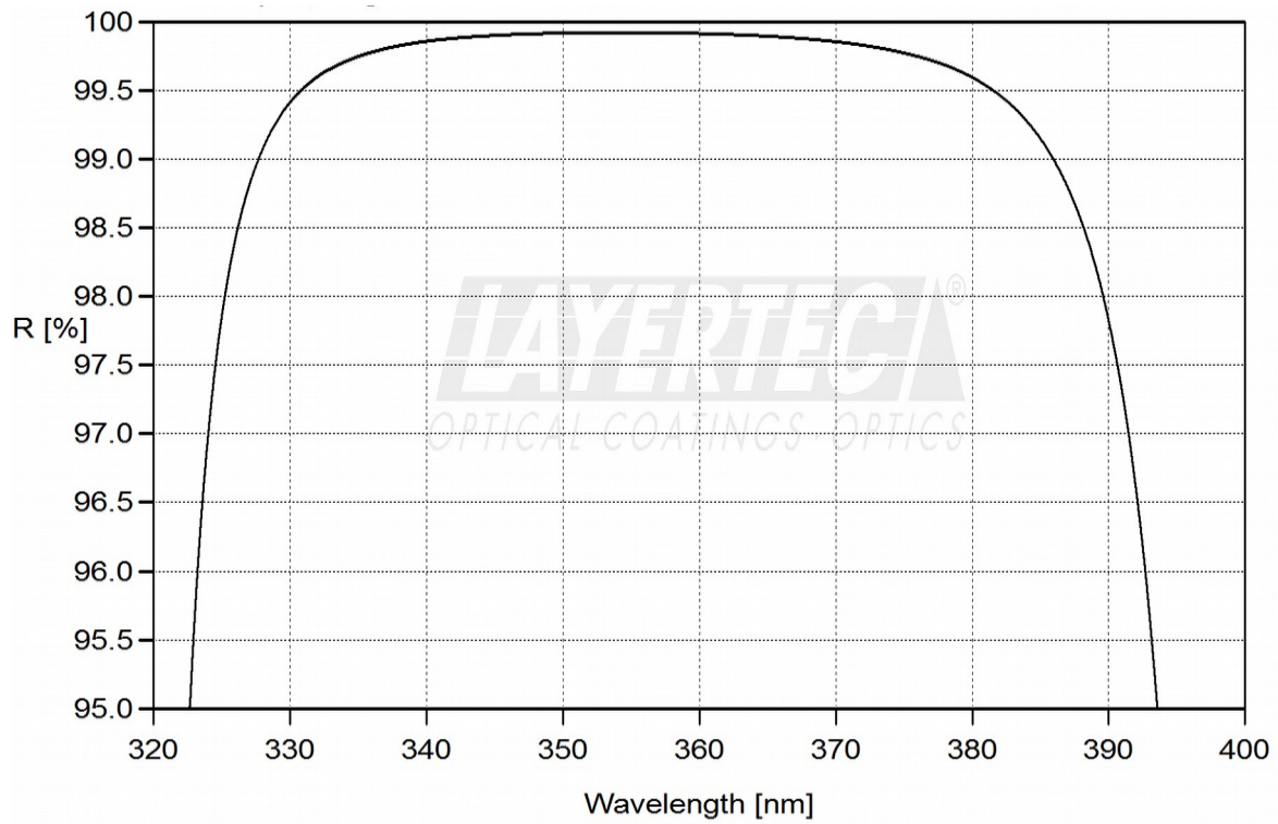
fig. 1.1: HR (0°, 355nm) > 99.5%
