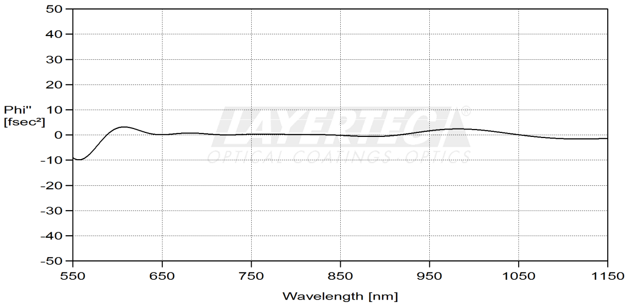
fig. 4 calculated GDD(T,0°)
