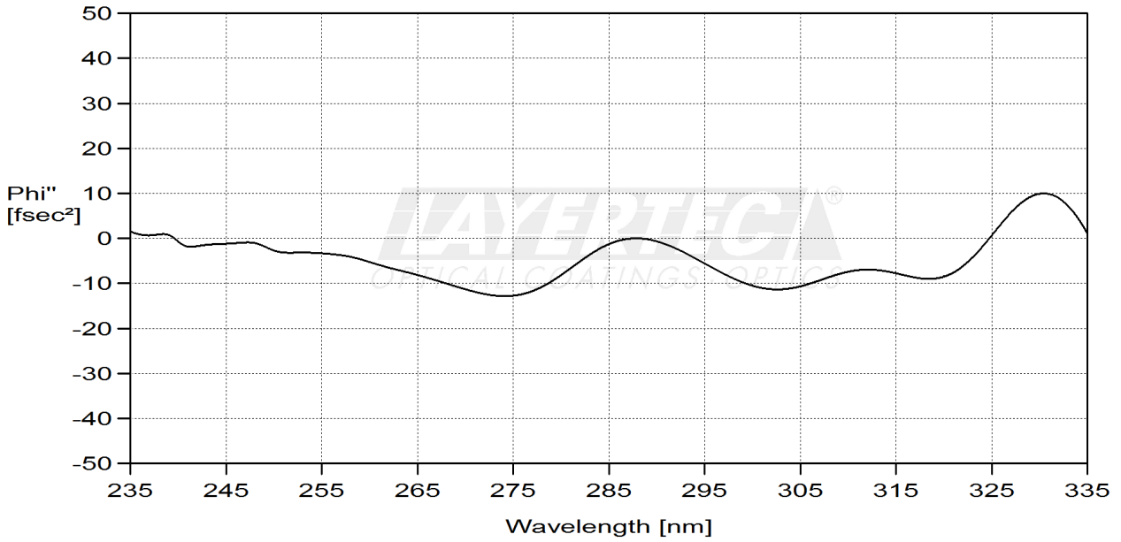
fig. 3 calculated GDD(R,0°)
