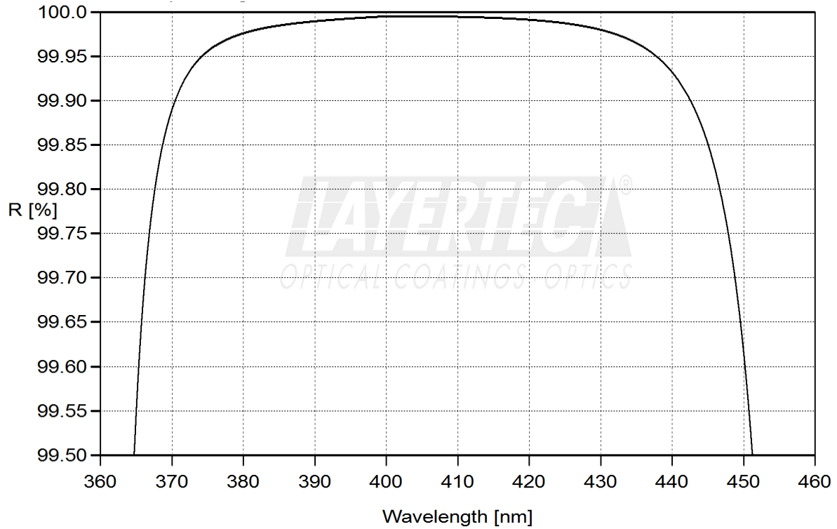
fig. 1.1: HR(0° 405nm)>99.98% T(0° 405nm)~0.005%
