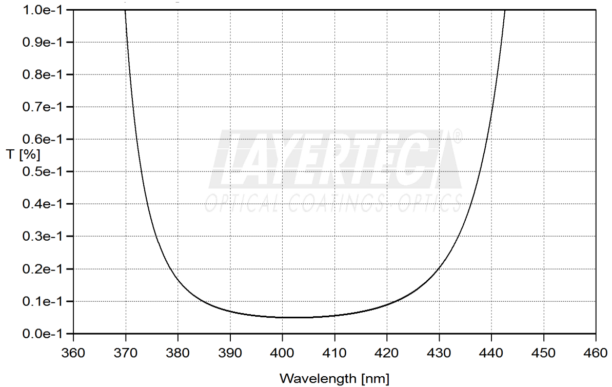
fig. 1.2: HR(0° 405nm)>99.98% T(0° 405nm)~0.005%
