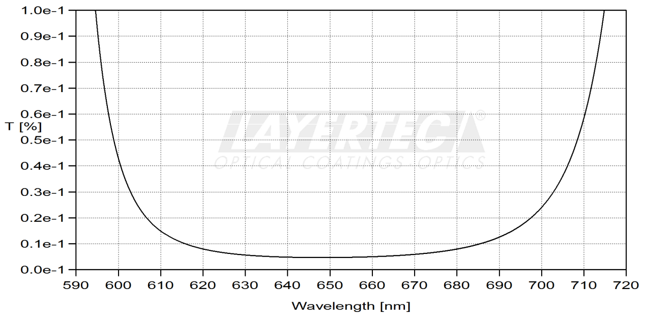
fig. 2 transmission PR-region 0°
