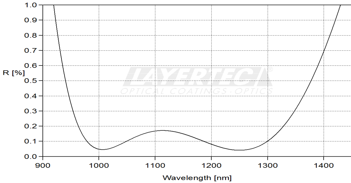
fig. 1 reflection AR 0°
