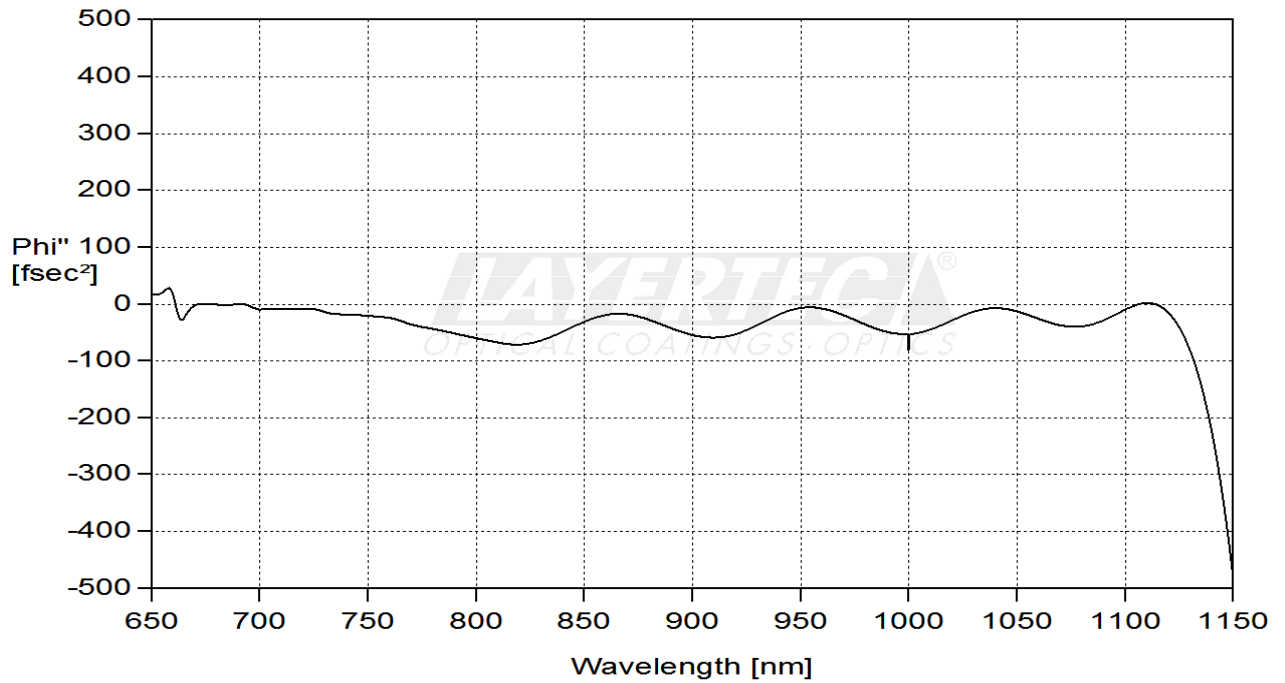
fig. 2 calculated GDD - reflection AOI 0°
