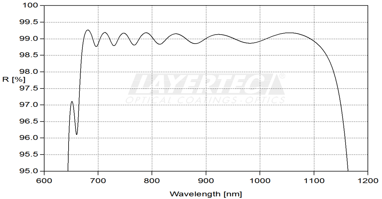
fig. 1 calculated reflection AOI 0°
