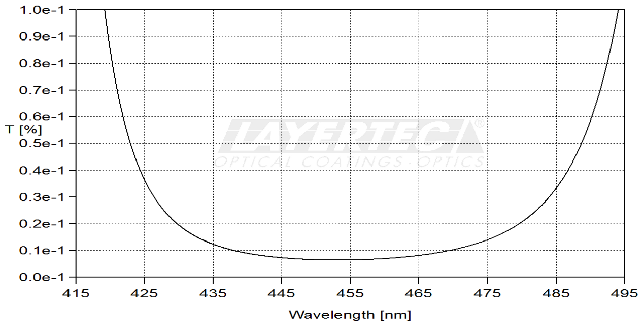
fig. 2 transmission HR-region 0°
