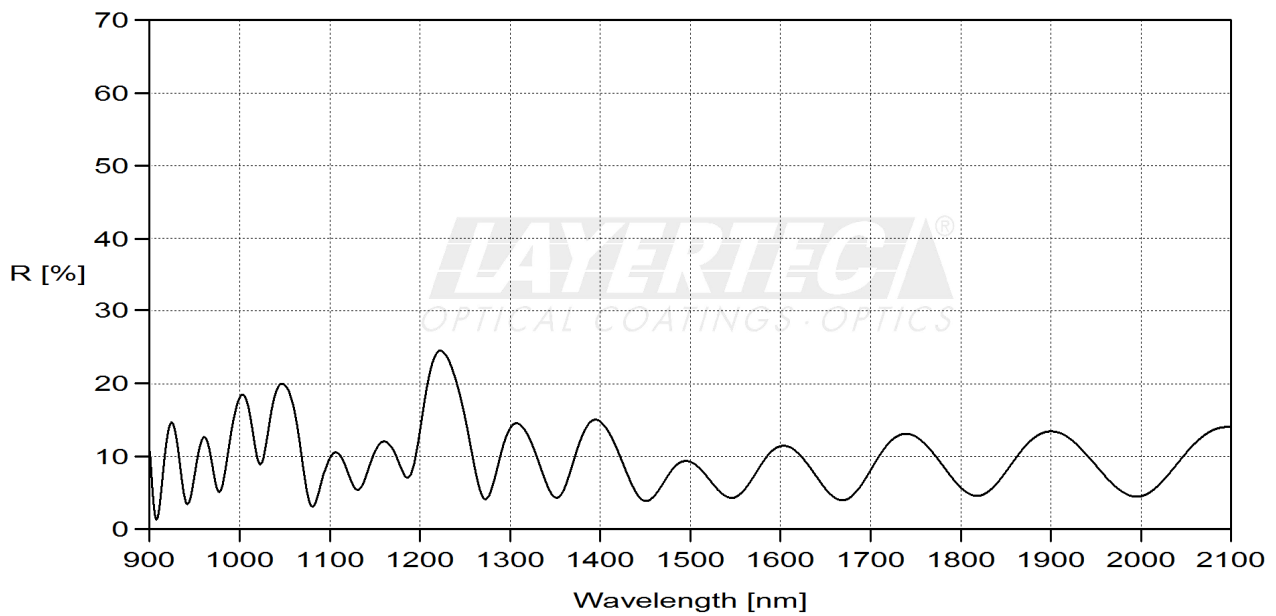
fig. 4 reflection HT-region 45° (unpolarised)
