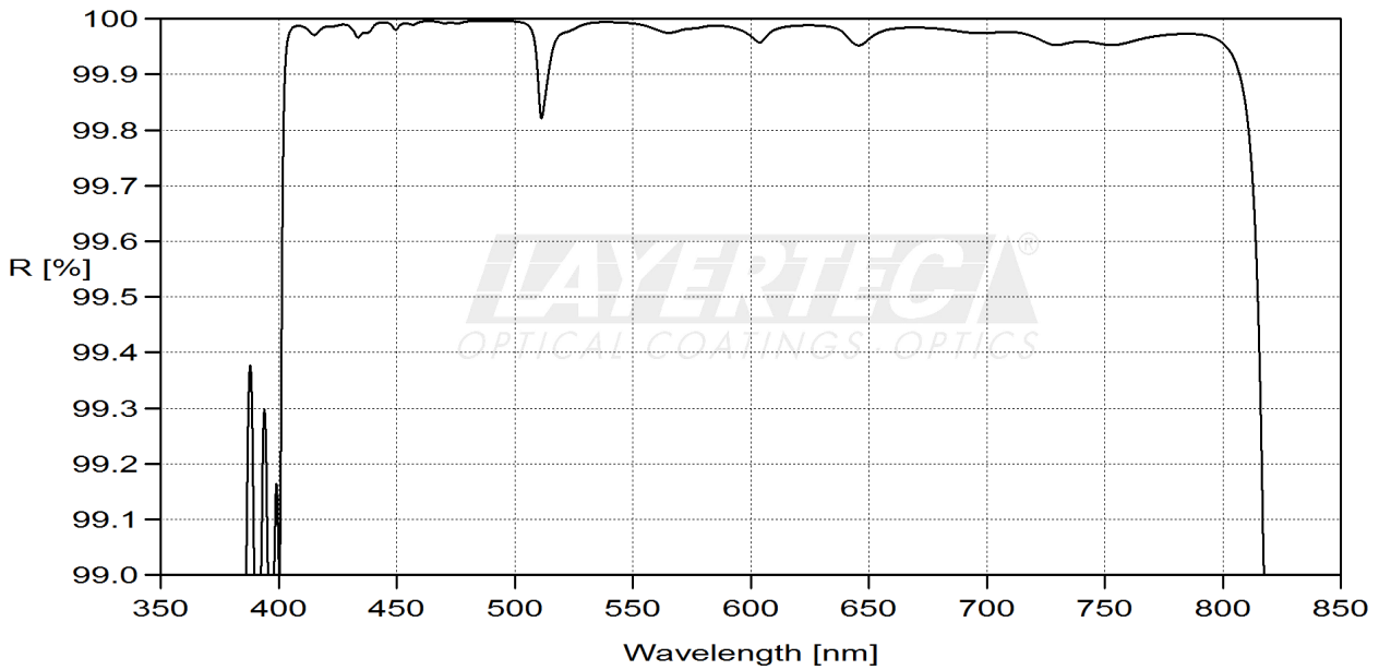
fig. 2 reflection HR-region 0°
