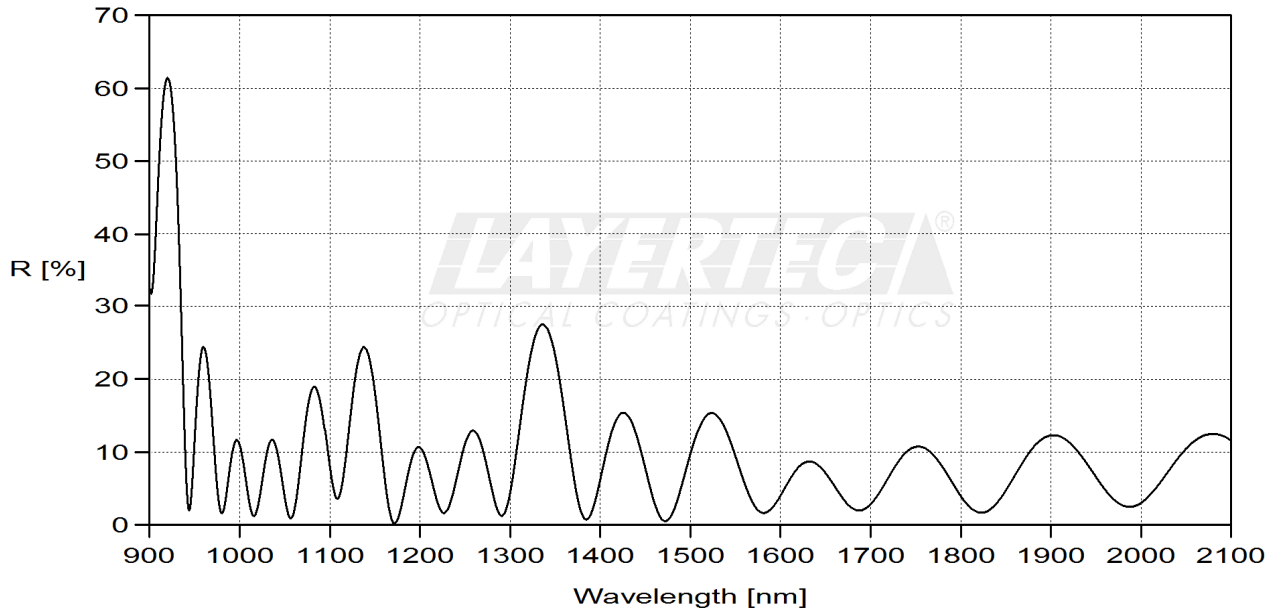
fig. 3 reflection HT-region 0°
