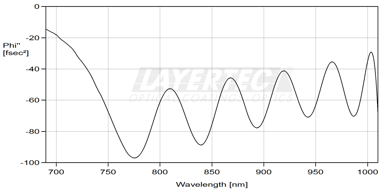
fig. 2 calculated GDD(R,0°)
