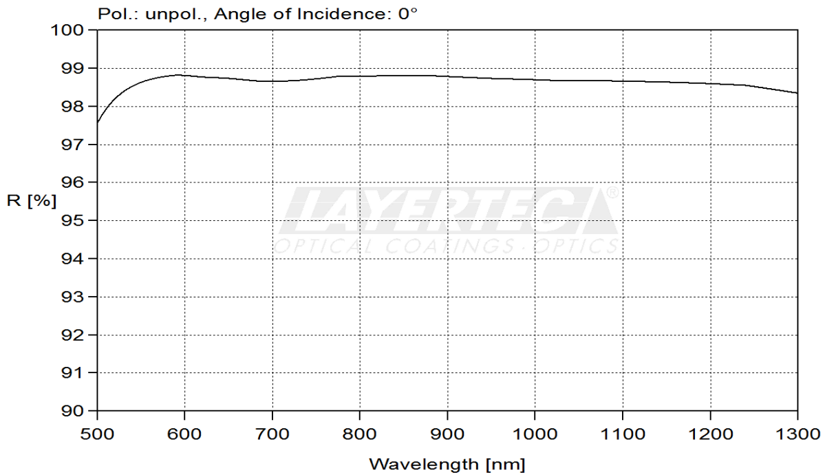
fig. 1 calculated reflectivity
