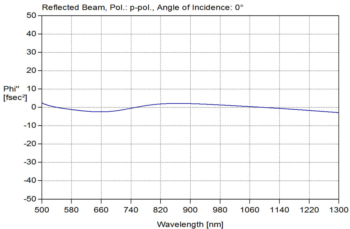
fig. 2 calculated GDD
