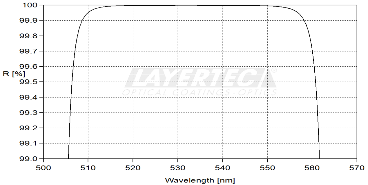
fig. 1 reflection HR-regions 0°
