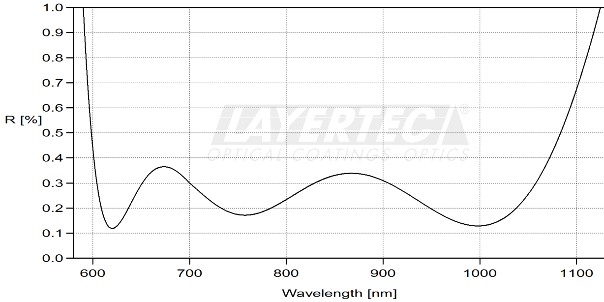
fig. 1 reflection AR 0°
