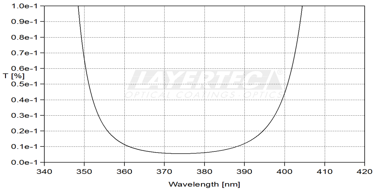
fig. 2 transmission HR-region 0°
