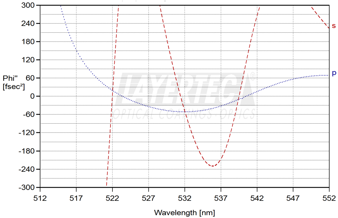
fig. 1.2: GDD – Rs,p at AOI = 45° at 532nm (not GDD opt.)
