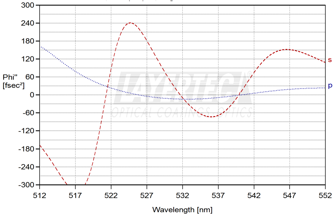
fig. 1.3: GDD – Ts,p at AOI = 45° at 532nm (not GDD opt.)
