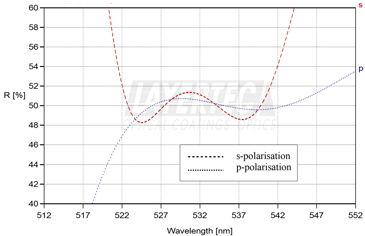
fig. 1.1: PR s,p (45° 532nm) = 50 ± 5% + |R s -R p | < 3%
