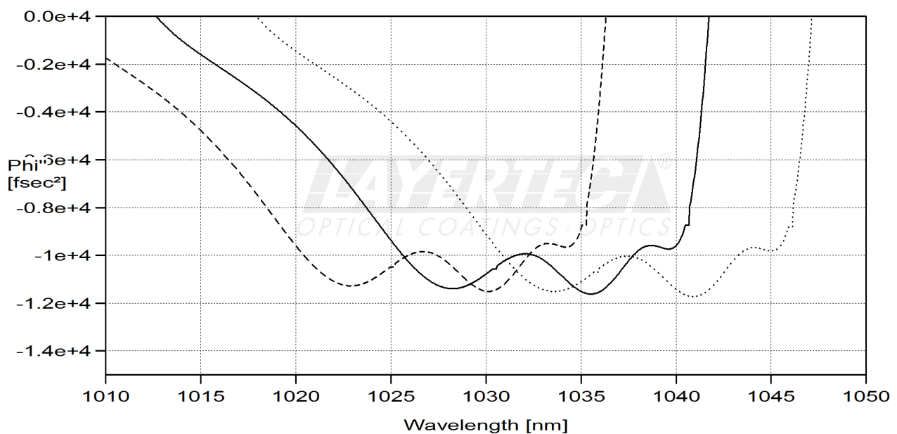
fig. 2 calculated GDD(R,0°) with typically shift \pm 5 nm of ZWL due to the production tolerance
