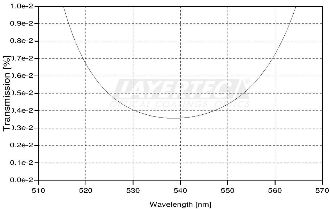
fig. 1: calculated transmission
