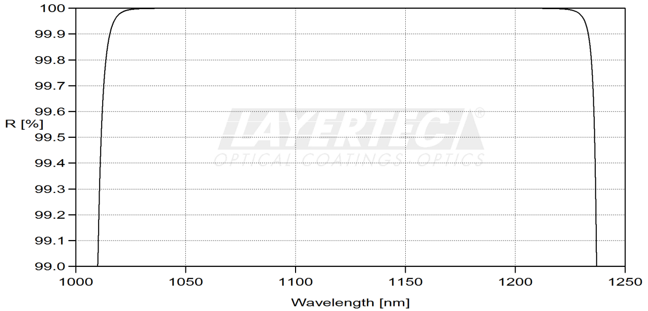
fig. 1 reflection HR-region 22.5° (unpolarized)
