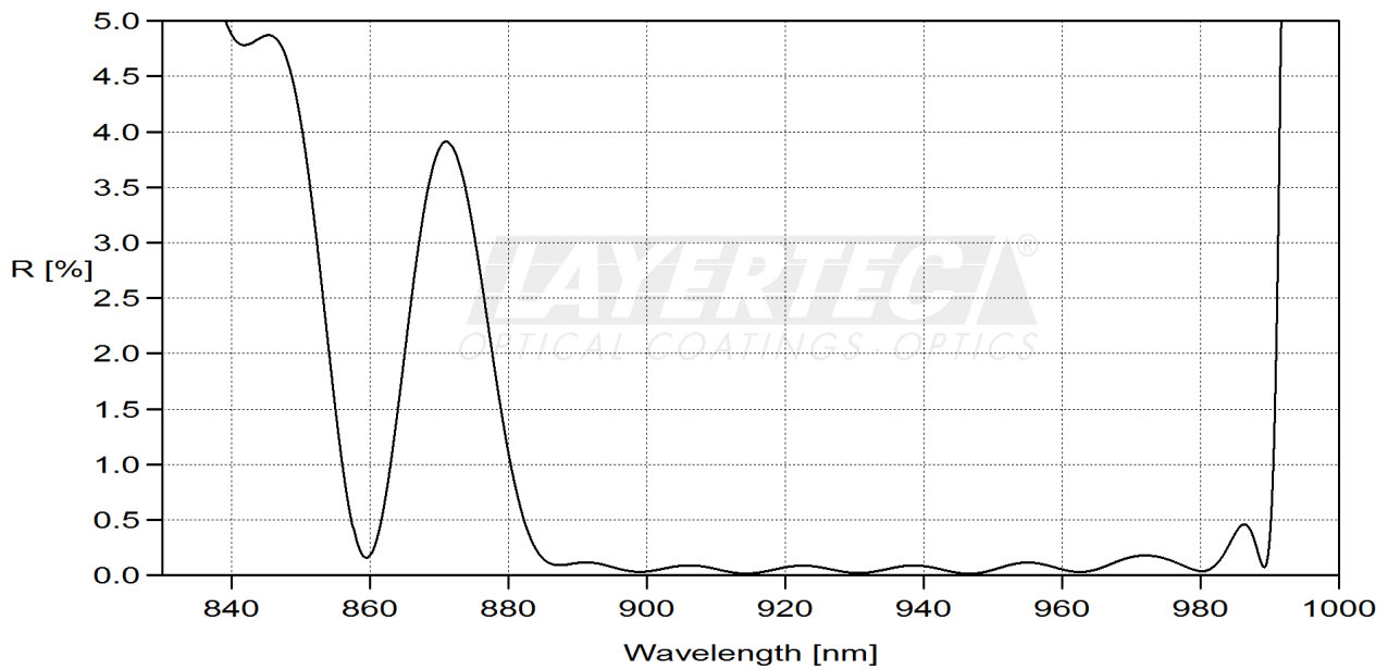
fig. 2 reflection R-region 22.5° (unpolarized)
