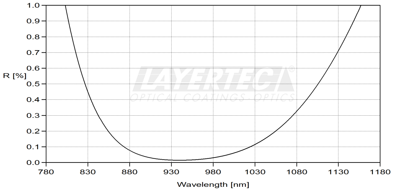
fig. 1 reflection AR 22.5° (unpolarized)
