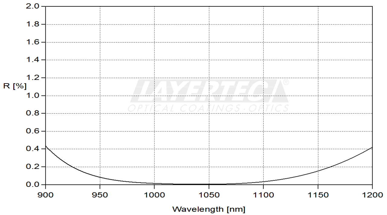
fig. 1 calculated reflection 0°
