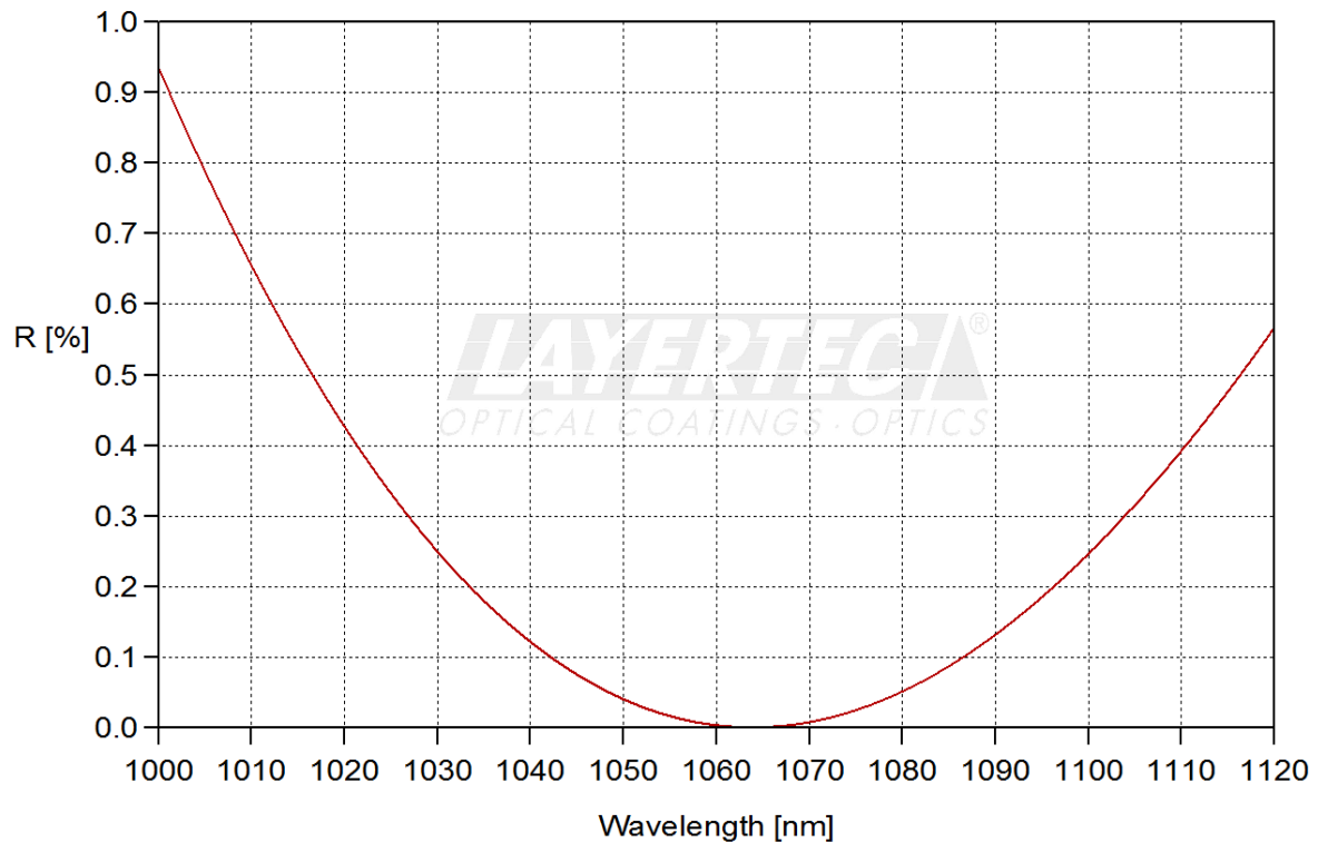
fig. 1.2: ARs (45° 1064nm) <0.5%
