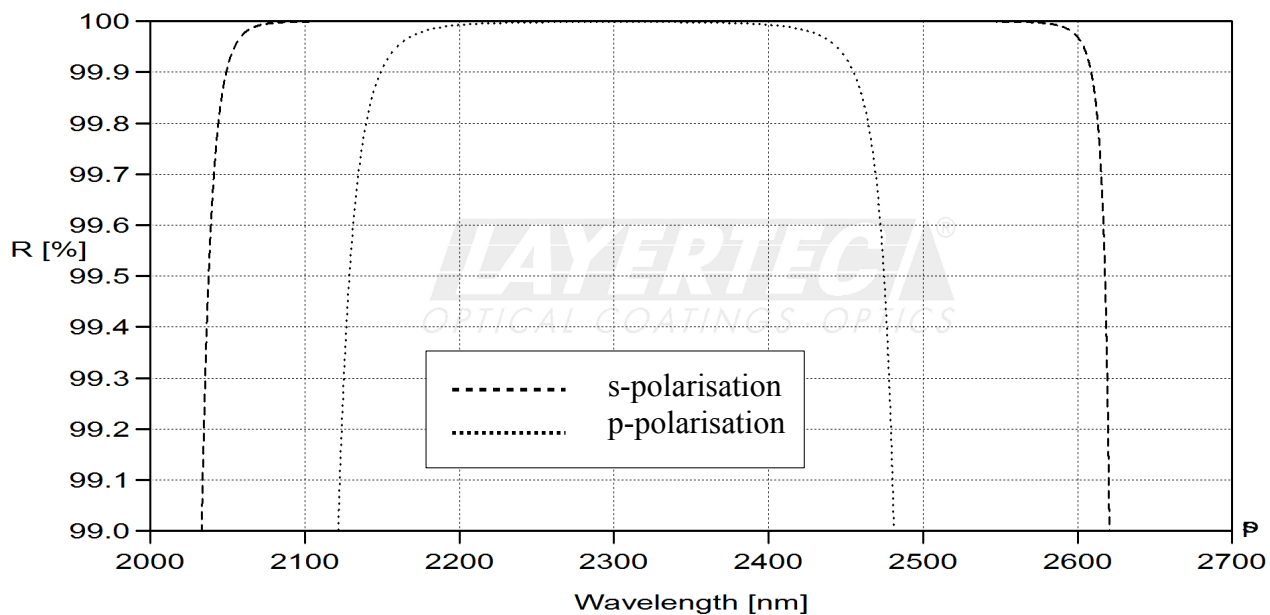
fig. 2 reflection R-region 45°
