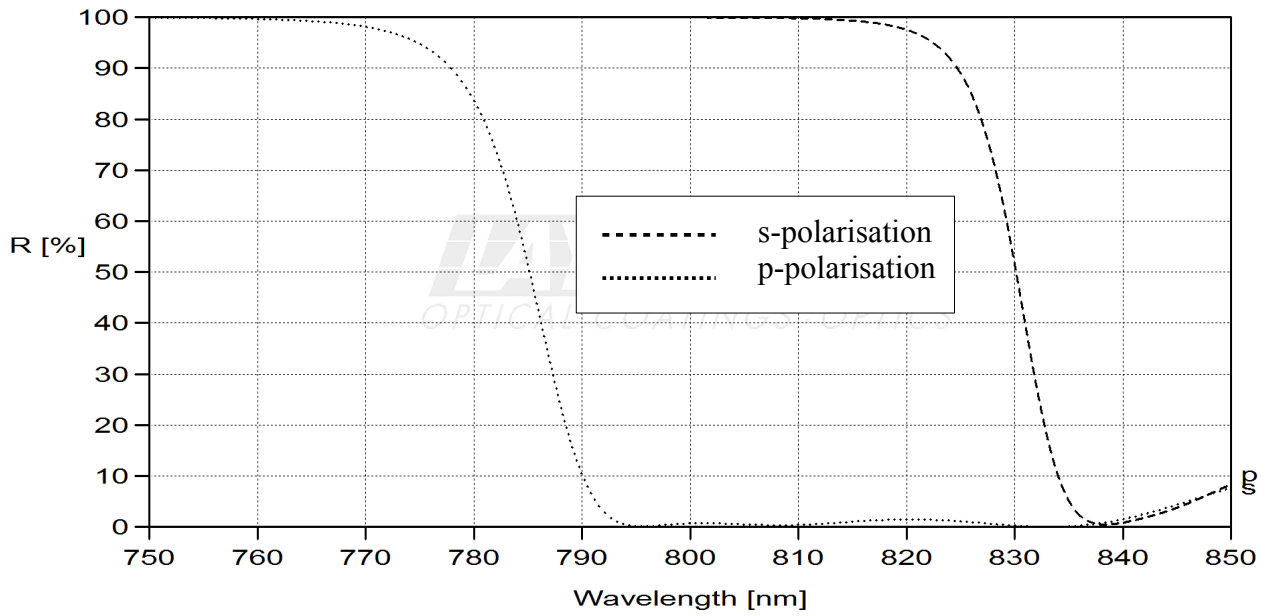
fig. 1 reflection for p- and s-polarisation for AOI=45°
