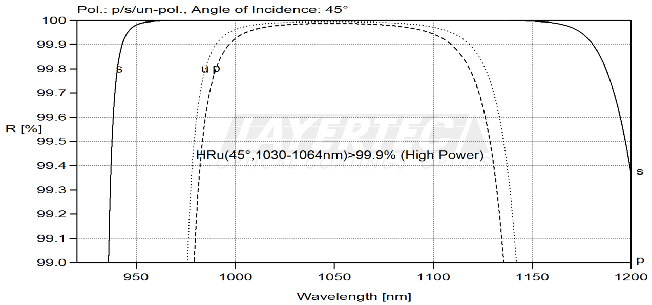
fig. 1 reflection, 45°
