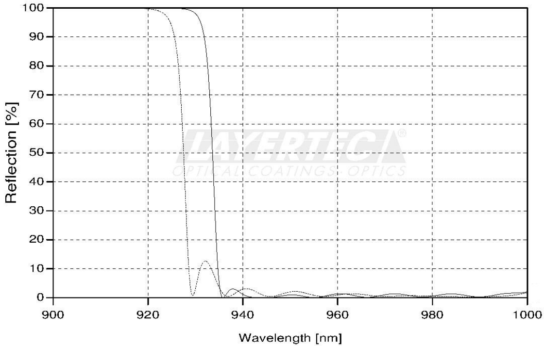
fig. 2: calculated reflectivity for AOI=45° “___” s-pol., “-----” p-pol., HR-region
