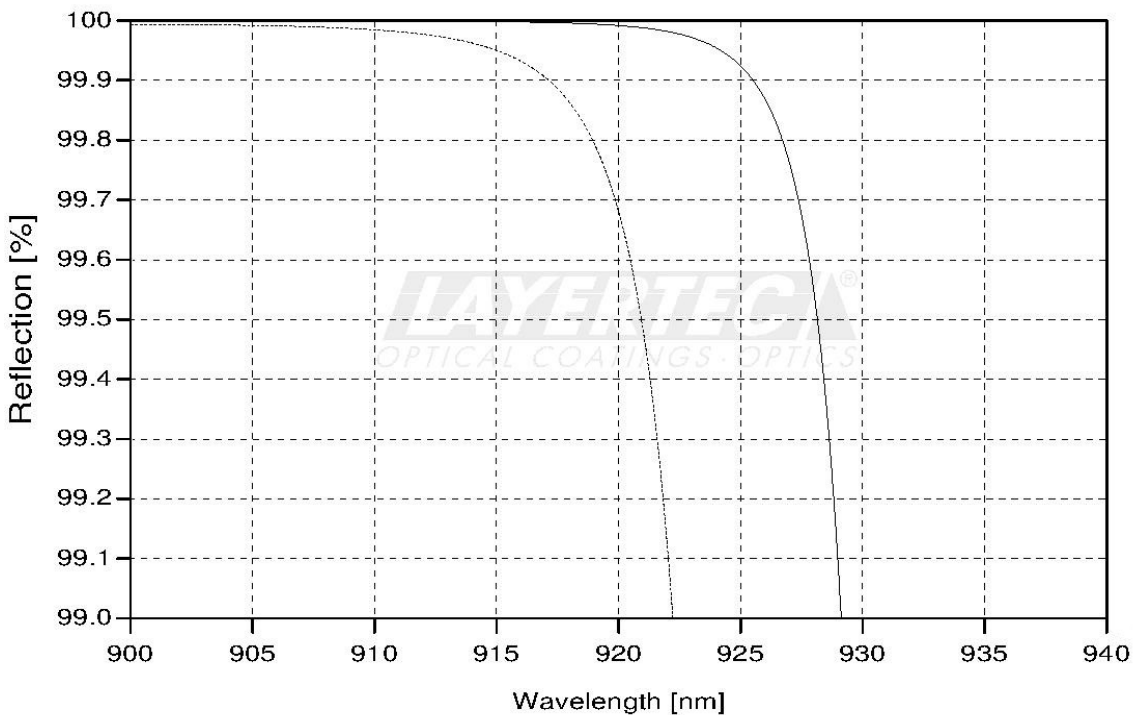
fig. 2: calculated reflectivity for AOI=45° “___” s-pol., “-----” p-pol., HR-region
