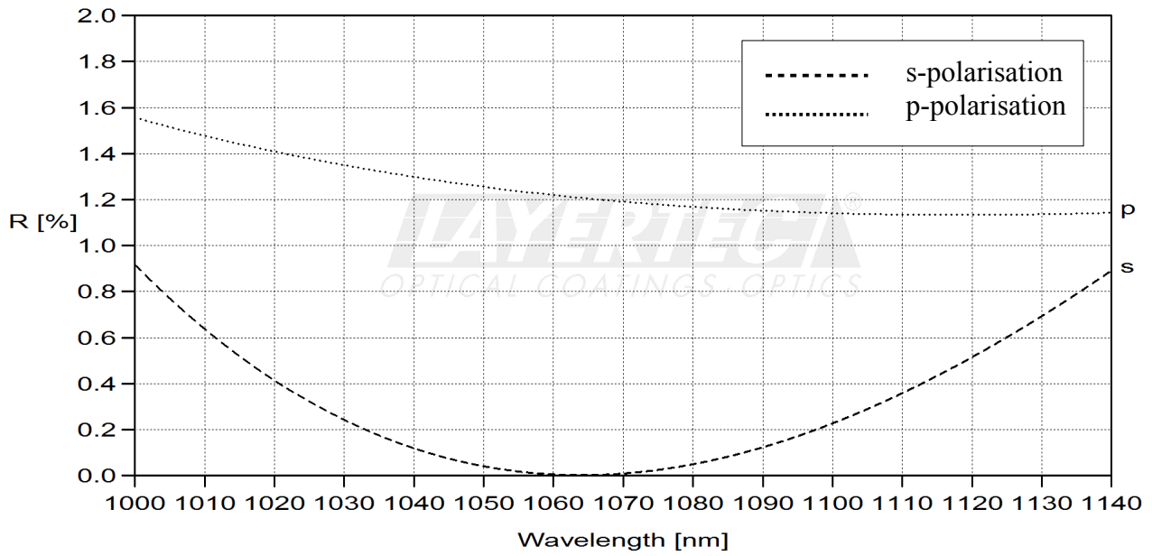
fig. 1 reflection AR 45°
