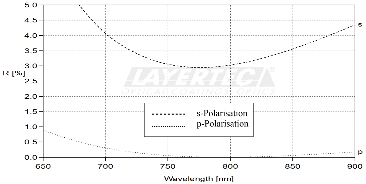
fig. 1 reflection AR 45°
