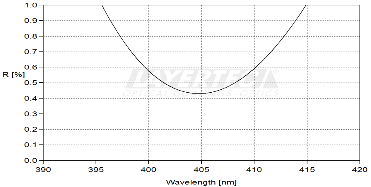
fig. 1 reflection AR 45° (unpolarised)
