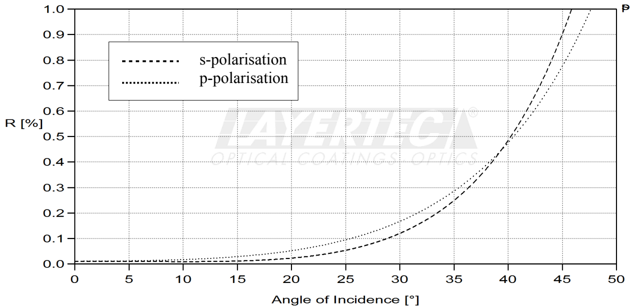
fig. 1 reflection versus AOI for \lambda = 1064\text{nm}
