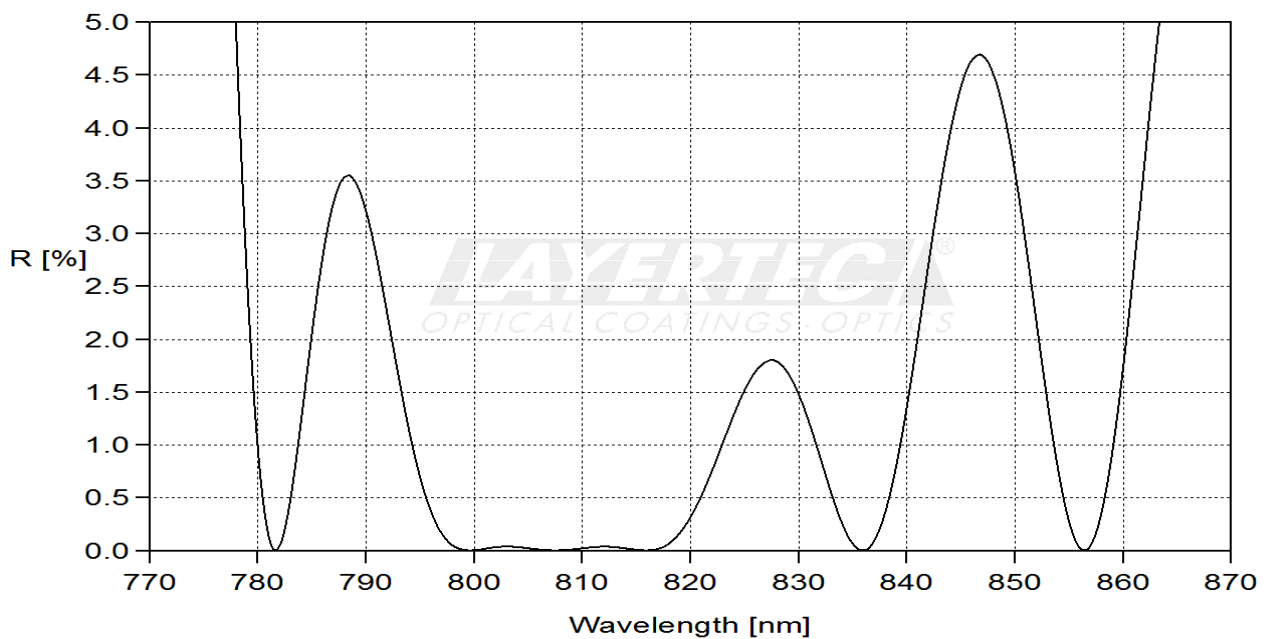
fig. 2 reflection R-region 0°
