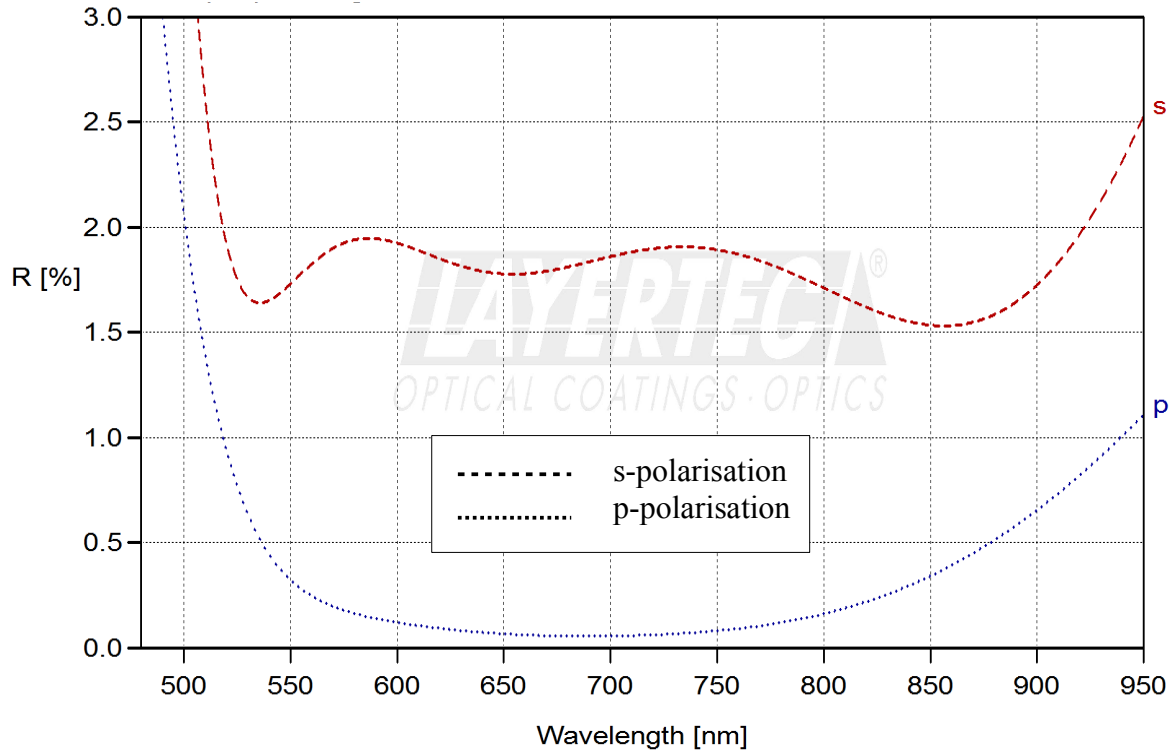
fig. 1.1: ARs(45°,520-900nm)<2% + ARp(45°,520-940nm)<1%
