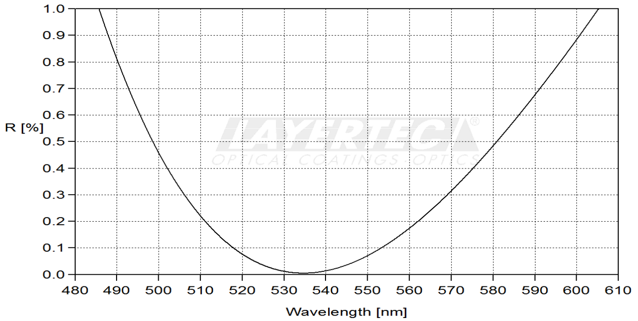
fig. 1 reflection AR 0°
