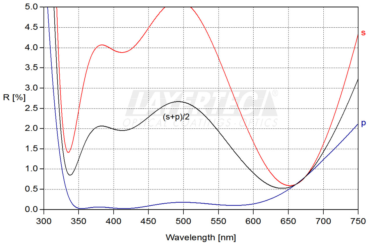
fig. 1 calculated reflection AOI 45° (without front side)
