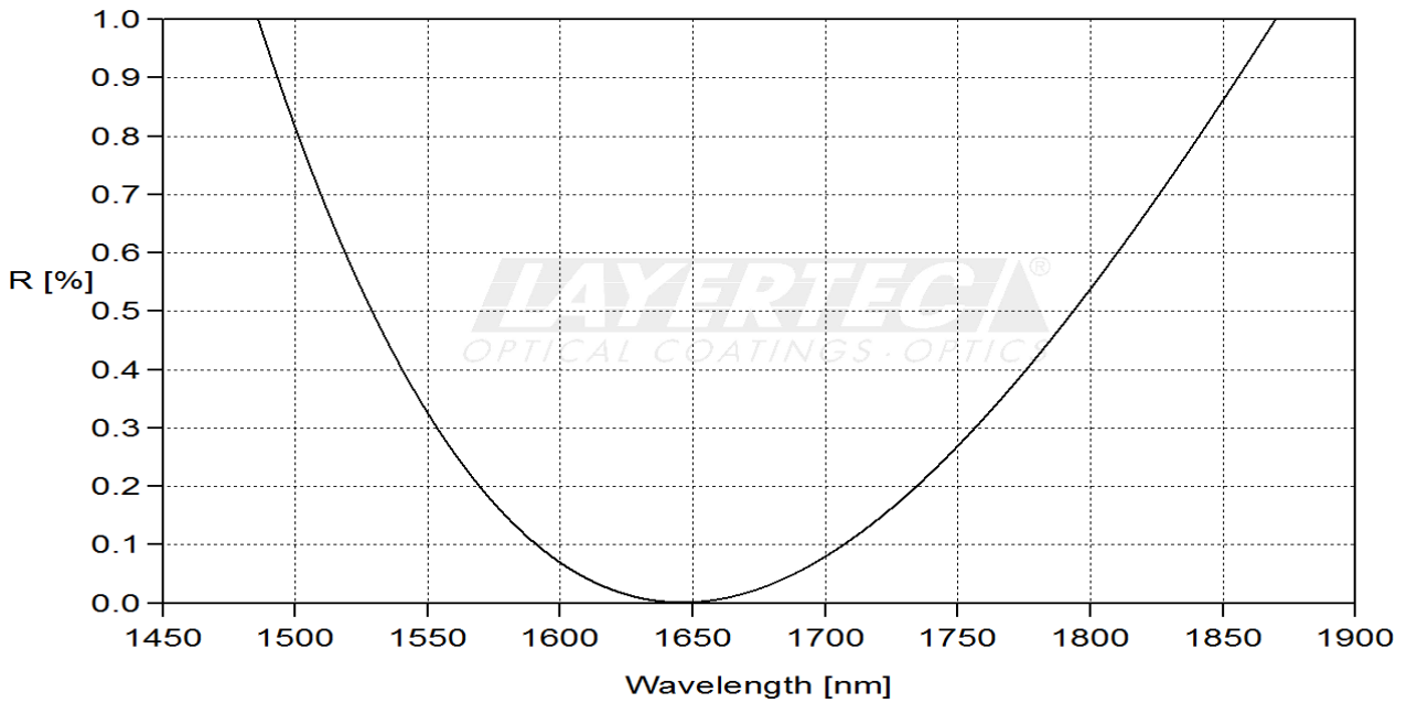
fig. 1 reflection AR 0°
