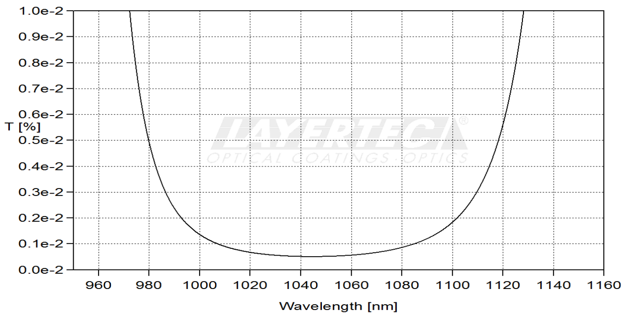
fig. 2 transmission HR-region 0°
