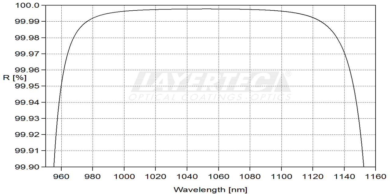
fig. 1 reflection HR-region 0°
