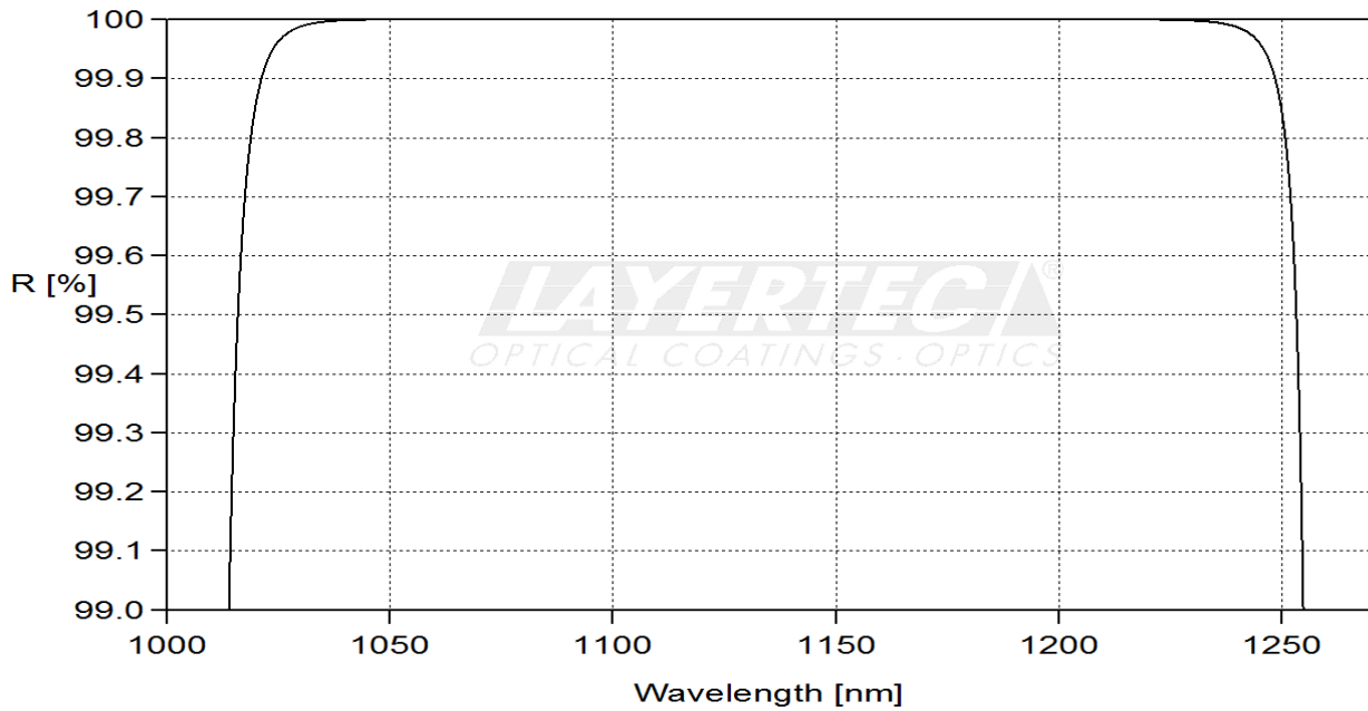
fig. 1 reflection HR-region 0°
