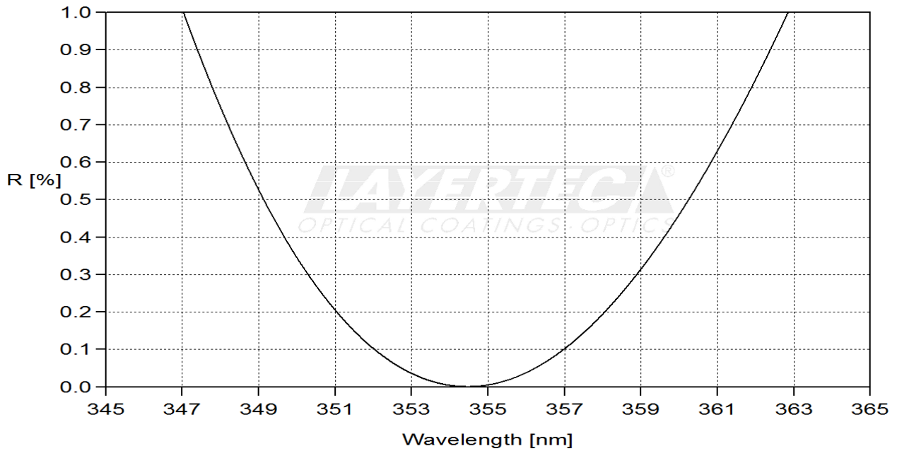
fig. 1 reflection AR 0°
