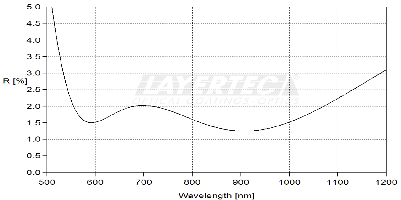
fig. 2 reflection AR 0°
