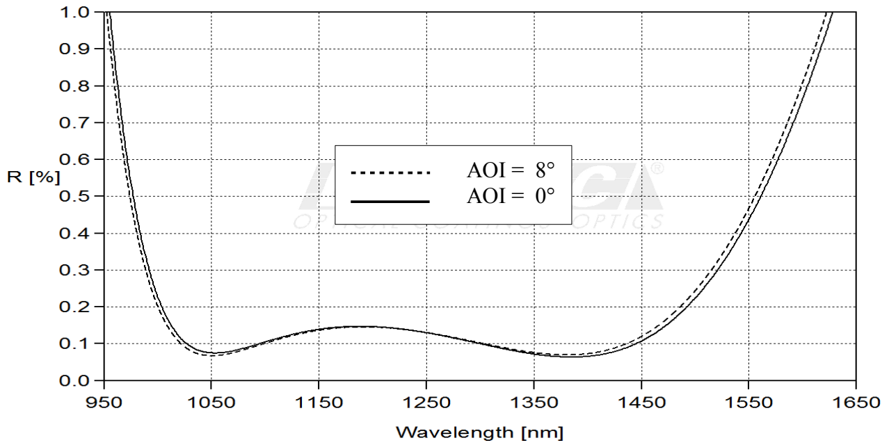
fig. 1 reflection AR (unpolarised)
