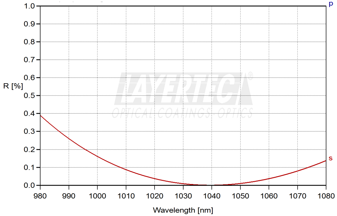
fig. 1.1: ARs (45°, 1020 - 1060nm) < 0.3%
