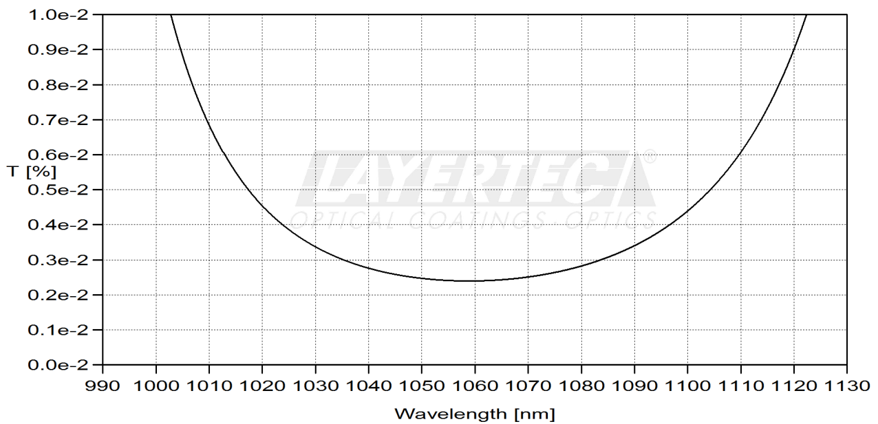
fig. 2 transmission HR-region 0°
