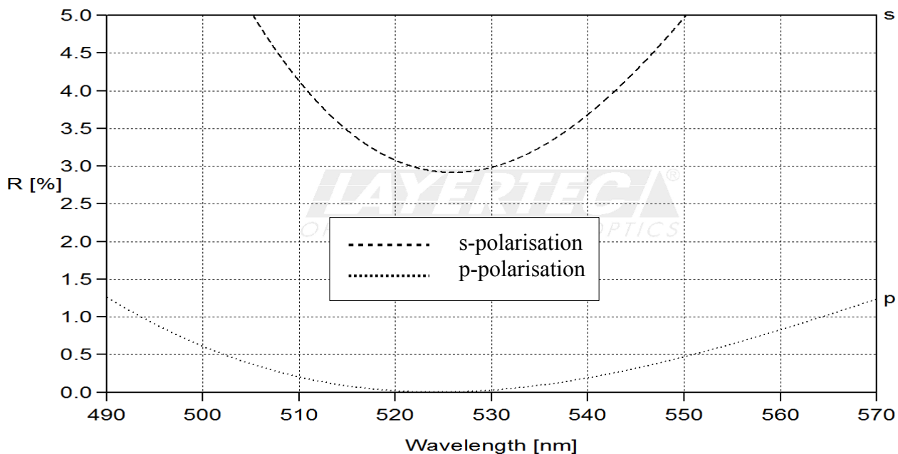
fig. 1 reflection AR 45°
