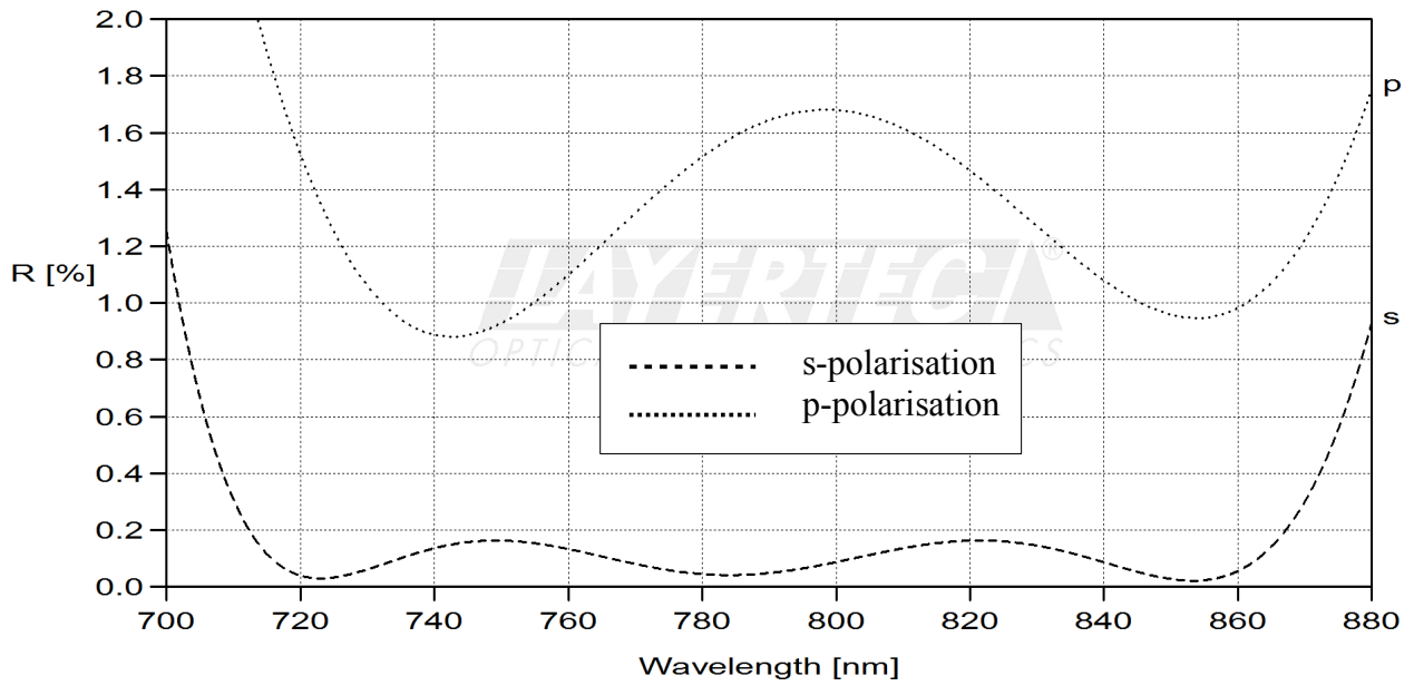
fig. 1 reflection AR 45°
