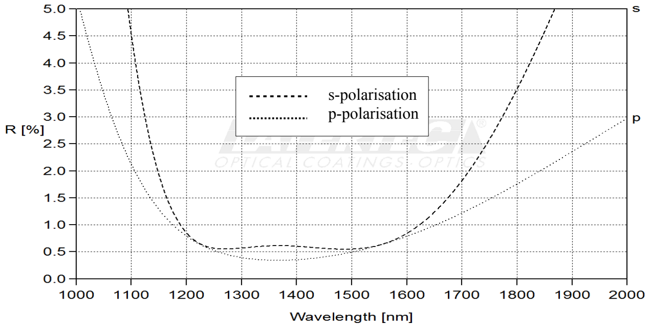
fig. 1 reflection AR 45°
