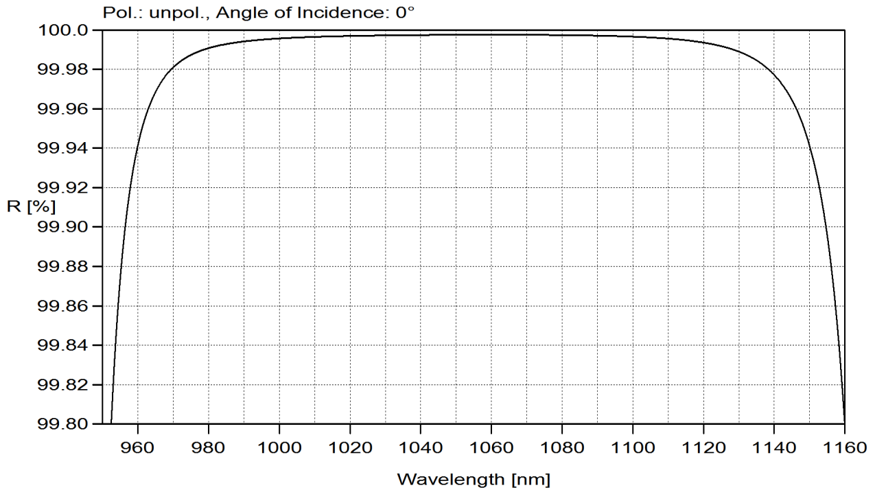
fig. 1 calculated reflectance
