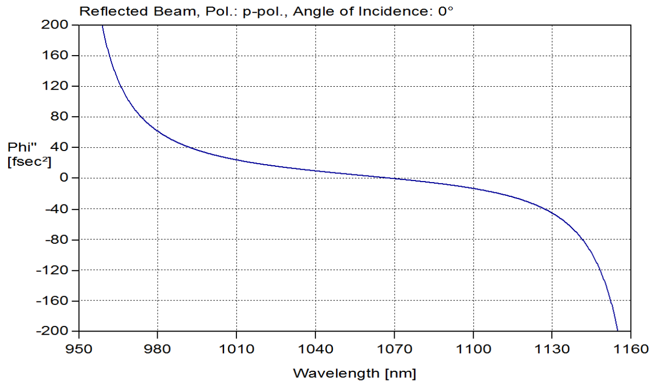
fig. 2 calculated GDD-R
