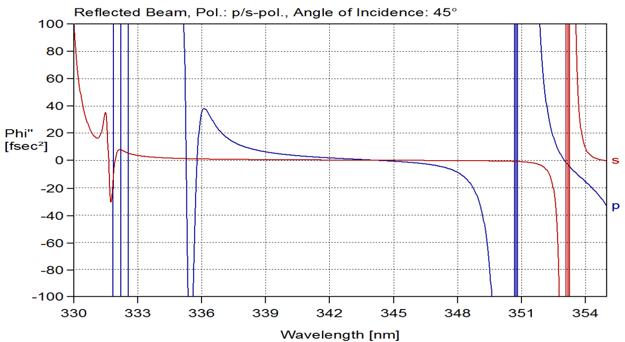
fig. 2 calculated GDD
