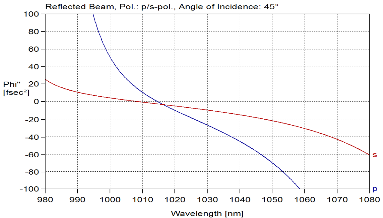
fig. 4 calculated GDD
