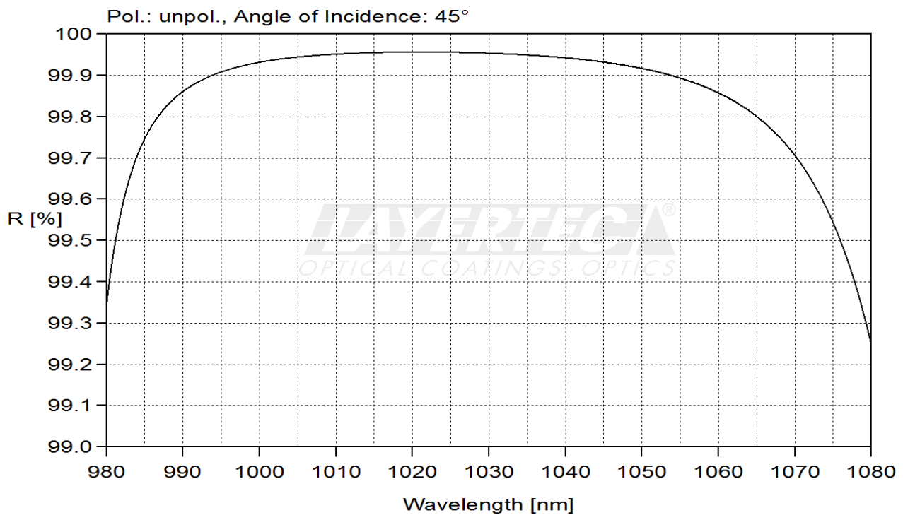
fig. 3 calculated reflectivity
