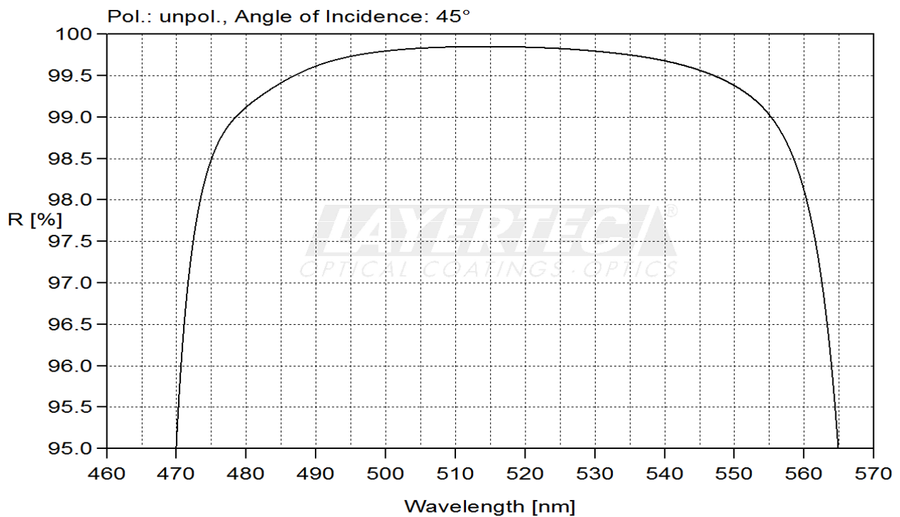
fig. 3 calculated reflectivity
