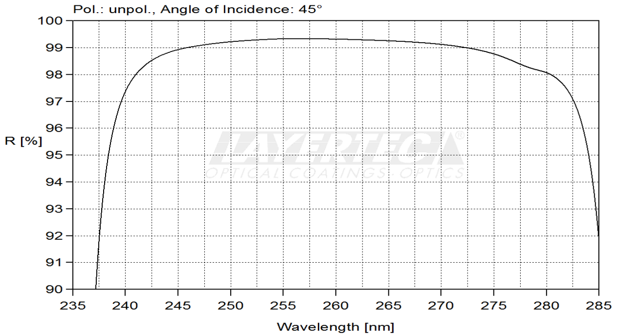
fig. 1 calculated reflectivity
