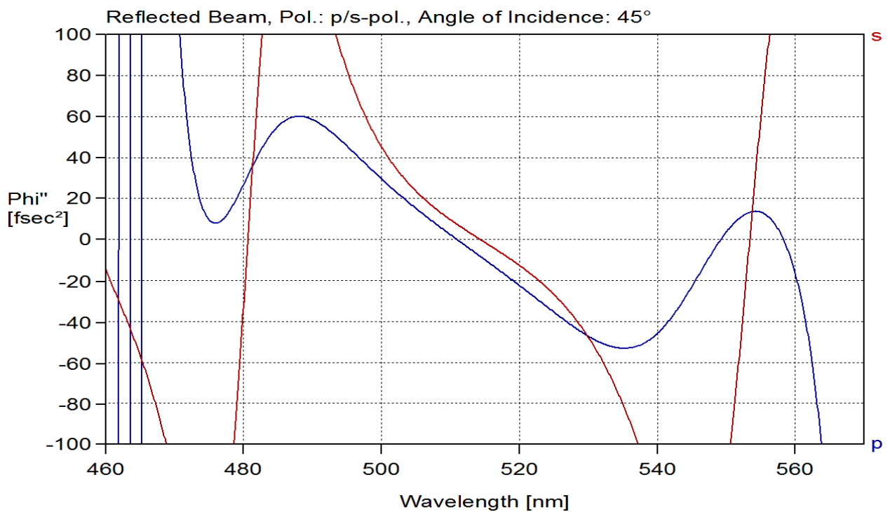
fig. 4 calculated GDD
