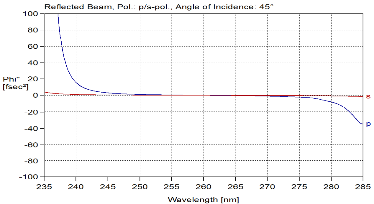
fig. 2 calculated GDD
