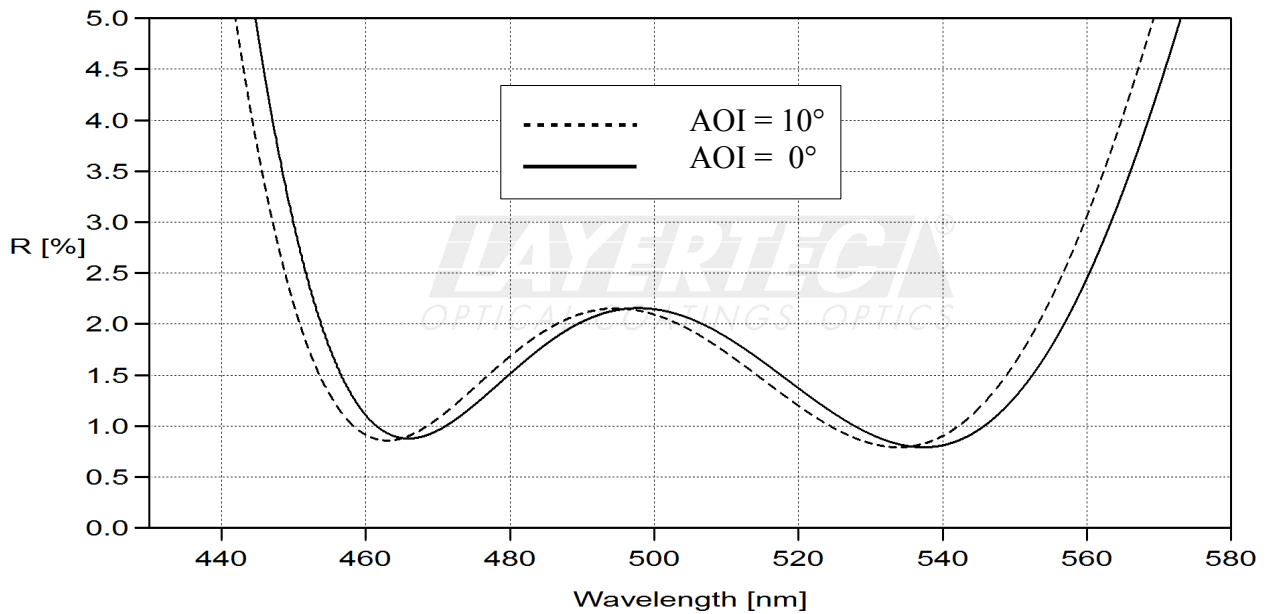
fig. 1 reflection AR (unpolarized)
